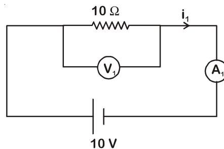
Circuit 1
