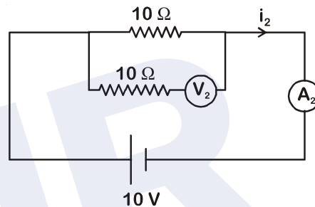
Circuit 2
